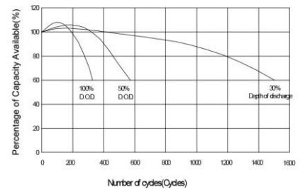
Number of cycles Vs. Depth of Discharge
