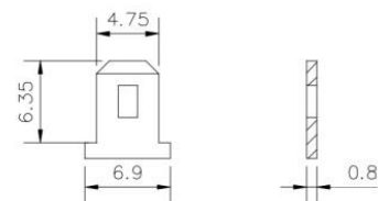
Standard Terminal Dimensions
